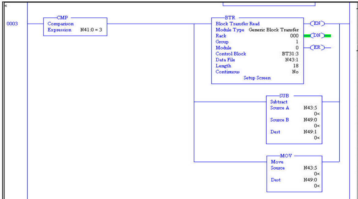
Figure 24: Ladder Logic Used to Collect the Change in Phase Match Error
