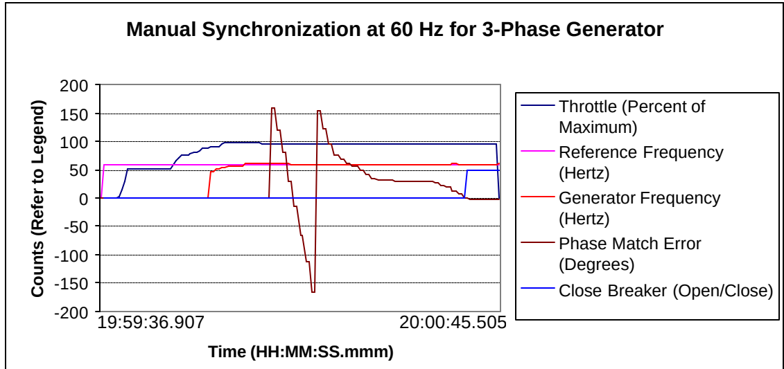
Figure 37: Manual Synchronization at 60 Hz for 3-Phase Generator
