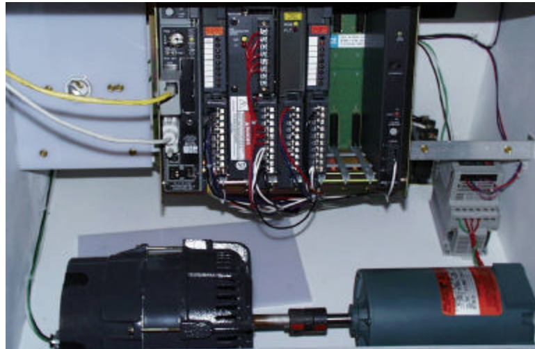
Figure 21: Wiring of the Generator Control System [11]
