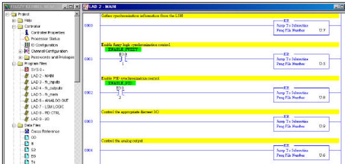
Figure 33: Ladder Logic Used to Switch Between Control Systems
