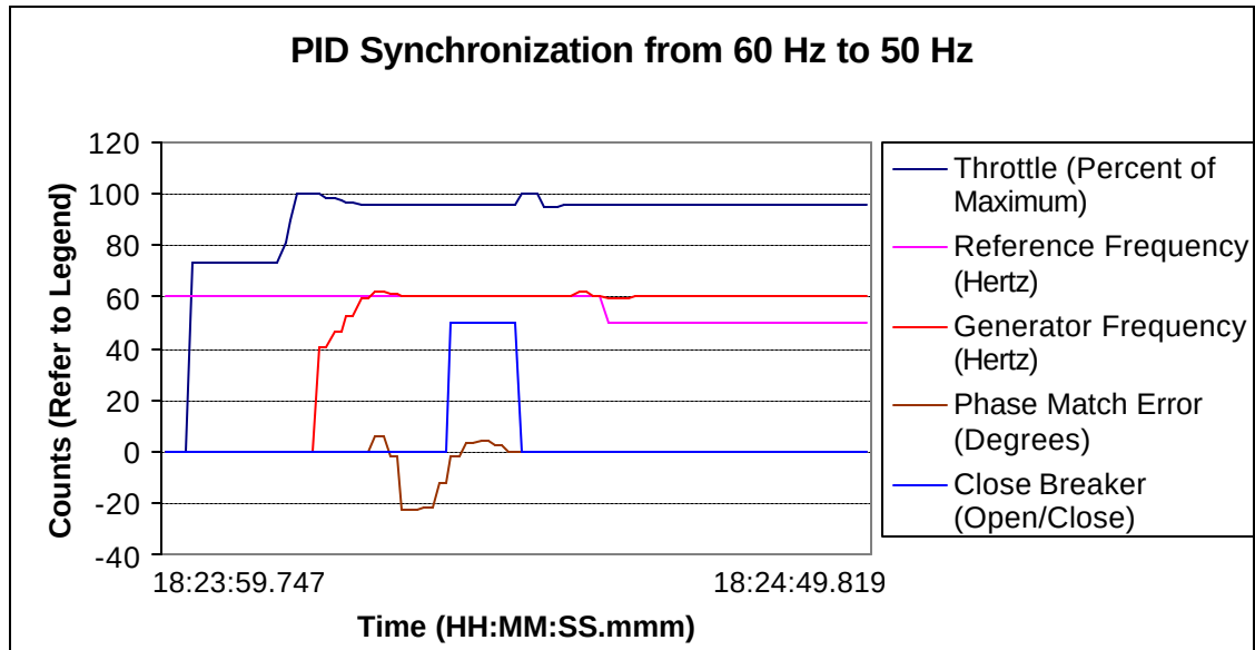
Figure 44: PID Synchronization from 60 Hz to 50 Hz
