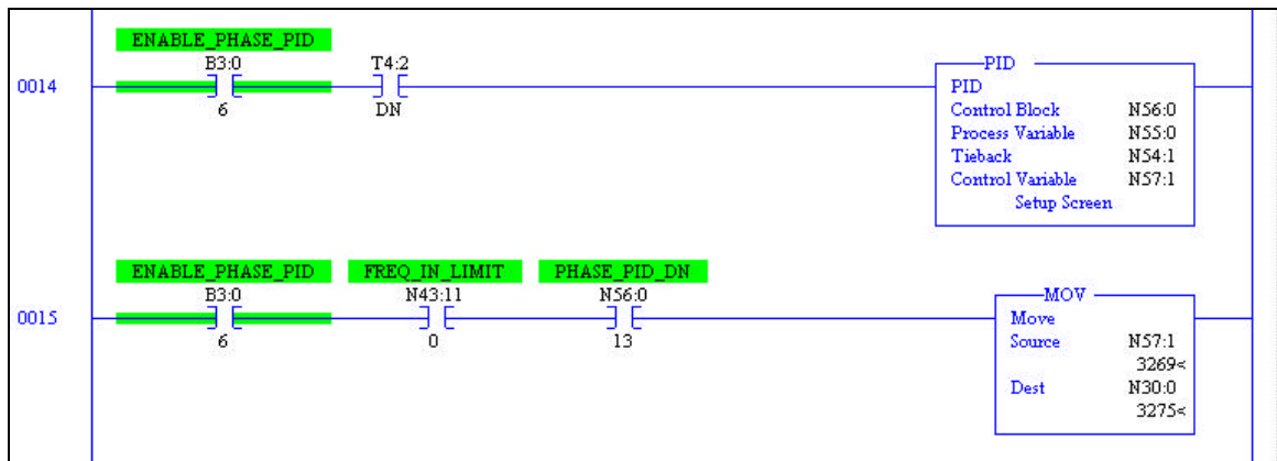
Figure 30: PID Loop Used to Synchronize Phase Angle
