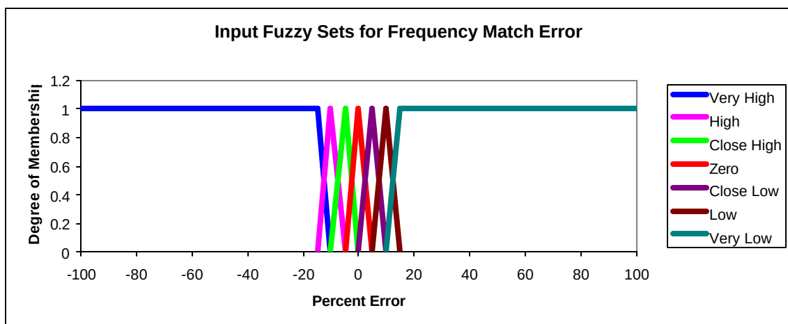
Figure 15: Input Fuzzy Sets for Frequency Match Error [11]
