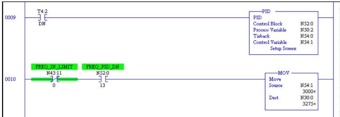
Figure 29: PID Loop used to Synchronize Frequency
