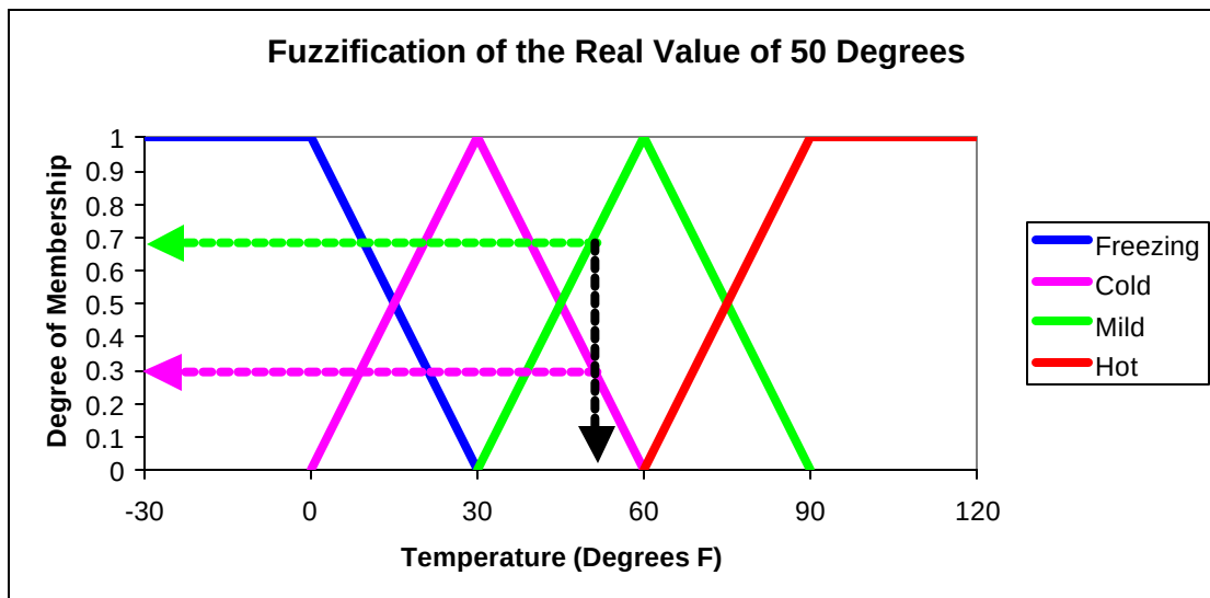
Figure 7: Fuzzification of a Real Value
