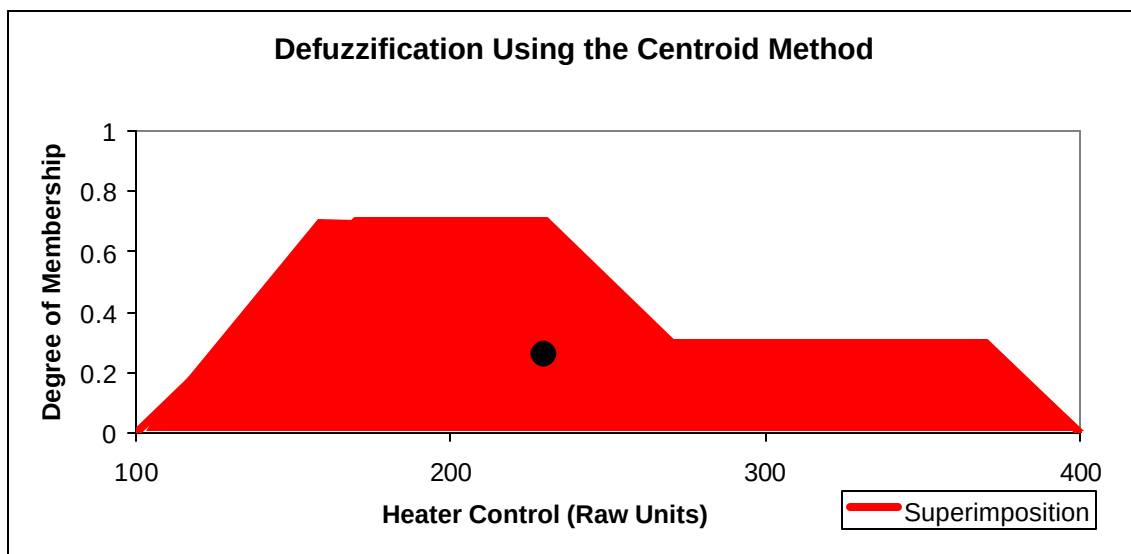
Figure 12: Defuzzification Using the Centroid Method
