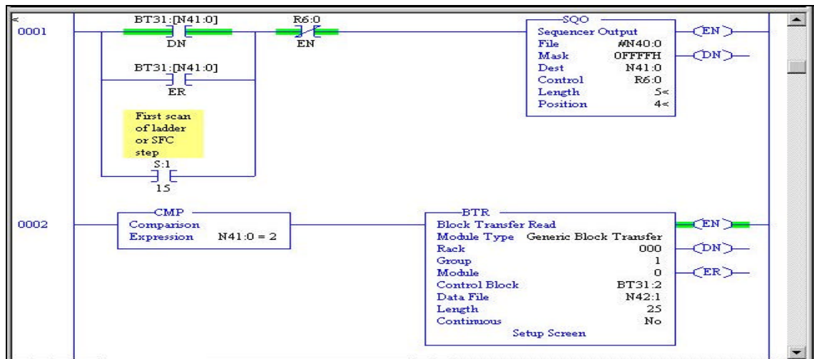
Figure 22: Ladder Logic for the Line Synchronization Module
