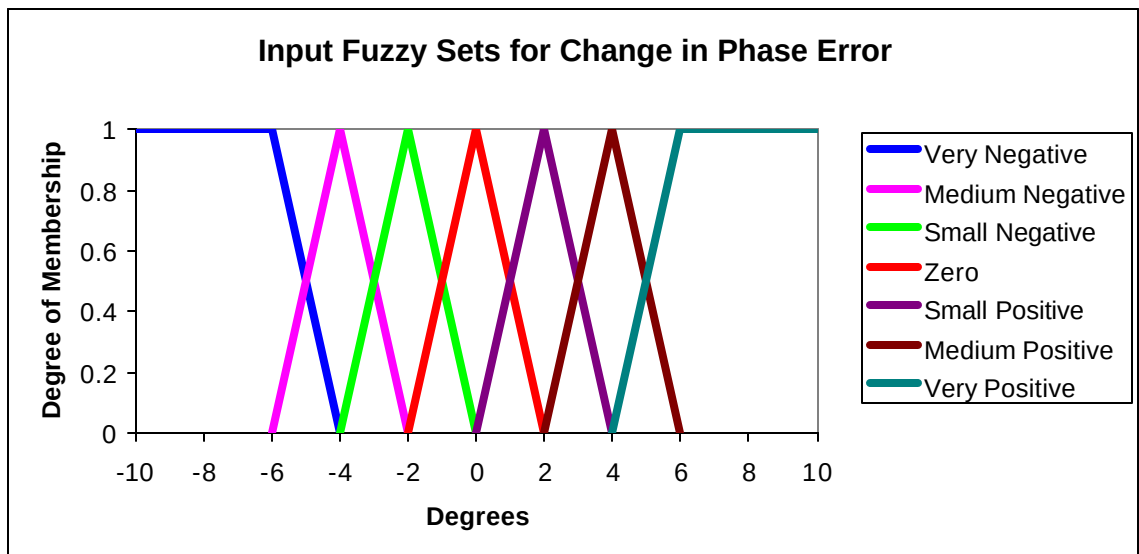
Figure 25: Input Fuzzy Set for Change in Phase Error
