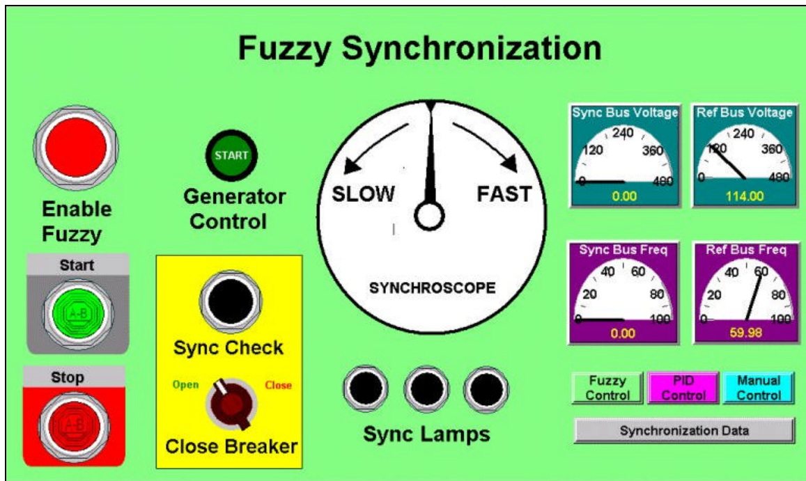
Figure 35: RSView32 Screen Used to Execute Fuzzy Logic Synchronization
