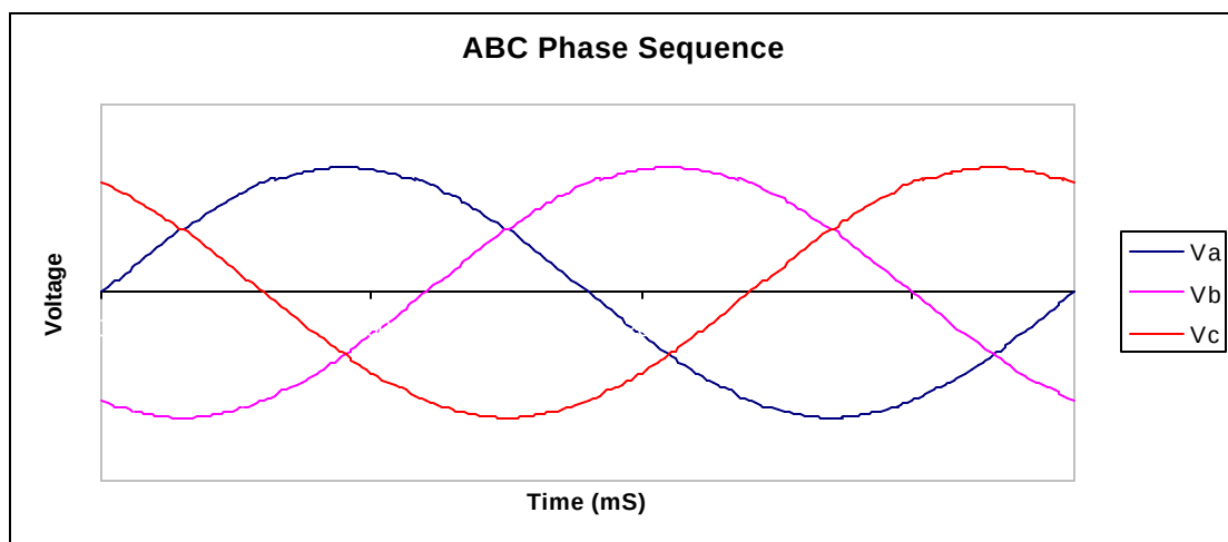
Figure 4: ABC Phase Sequence [1]
