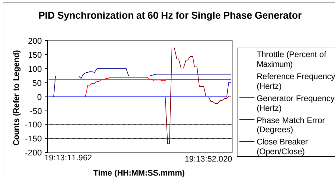
Figure 41: PID Synchronization at 60 Hz for Single-Phase Generator
