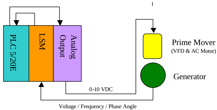
Figure 20: Diagram of the Generator Synchronization Control System
