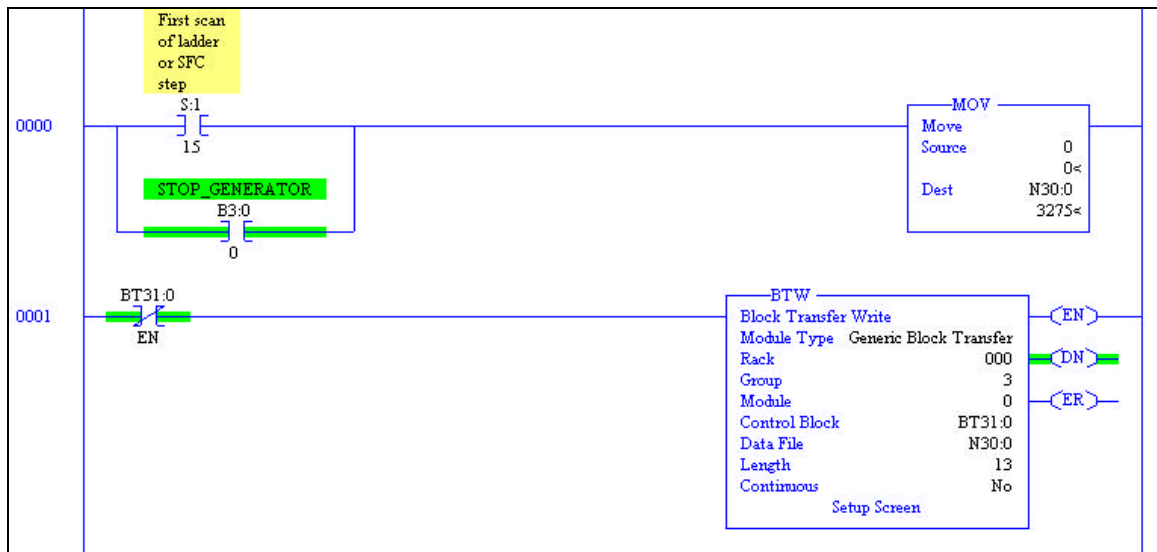
Figure 31: Ladder Logic Used to Change the Signal of the Analog Output Module
