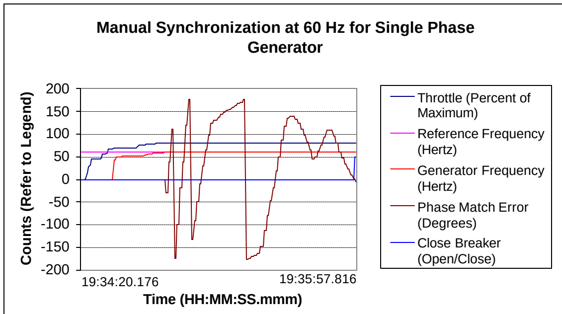
Figure 40: Manual Synchronization at 60 Hz for Single-Phase Generator
