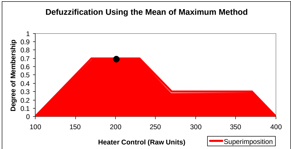
Figure 13: Defuzzification Using the Mean of Maximum Method
