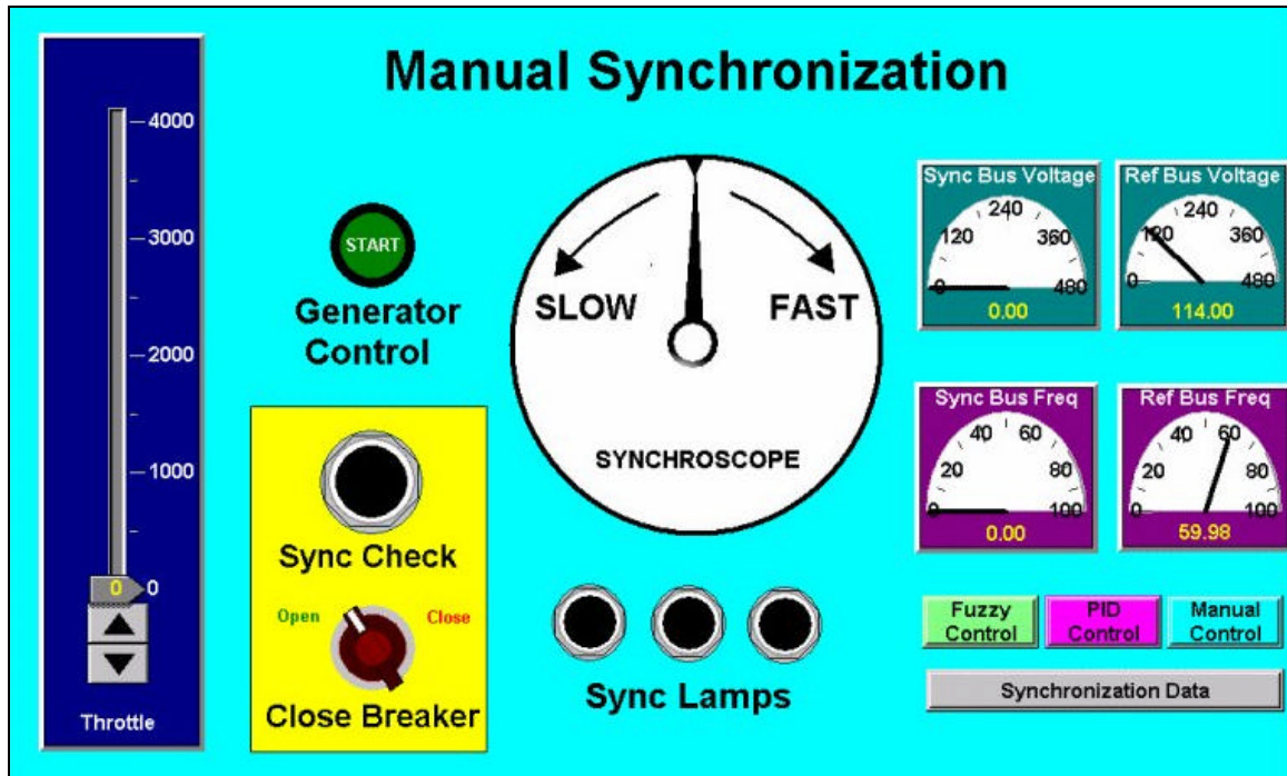
Figure 32: RSView32 Screen for Manual Synchronization
