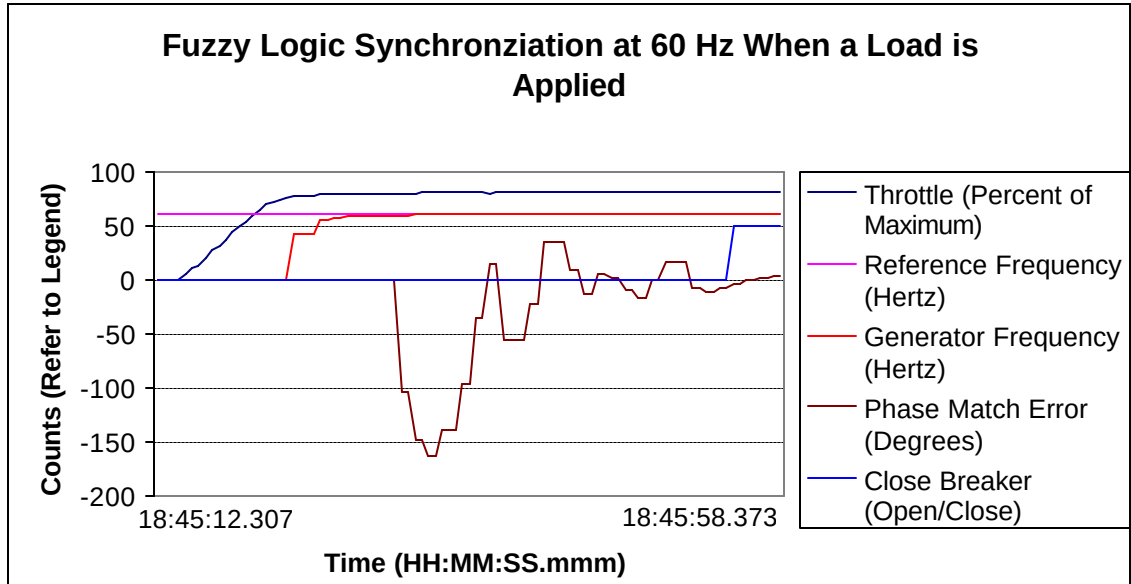
Figure 47: Fuzzy Logic Synchronziation at 60 Hz When a Load is Applied
