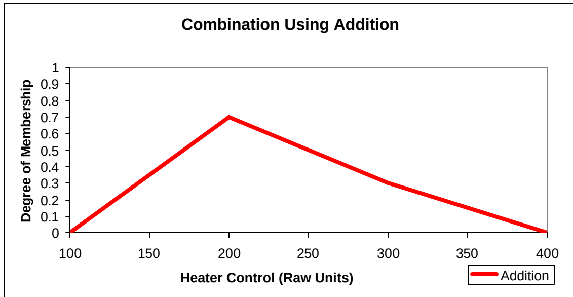
Figure 11: Combination Using Addition
