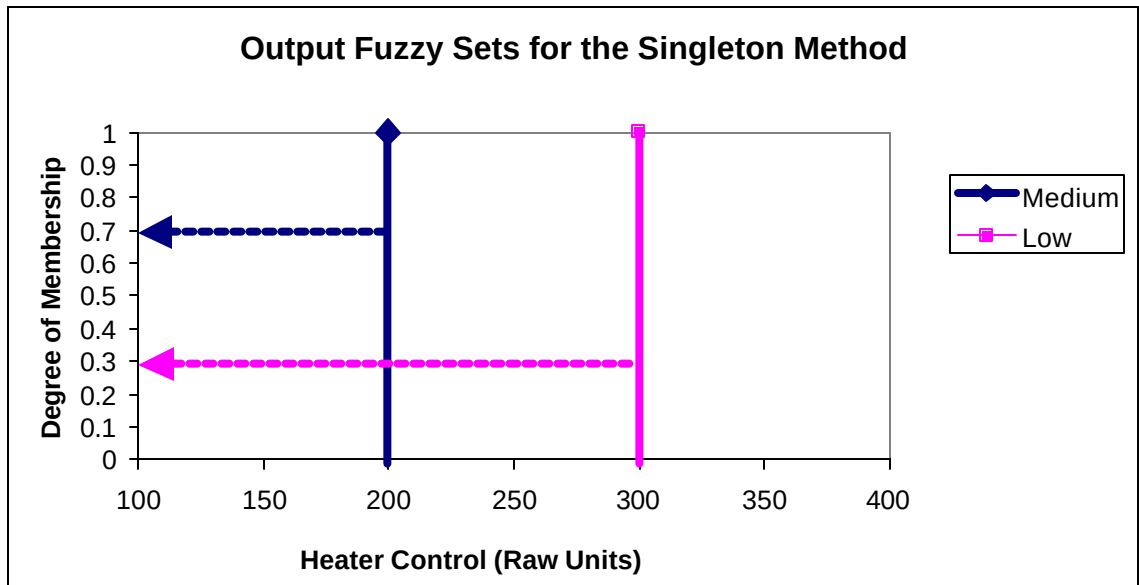
Figure 14: Output Fuzzy Sets for the Singleton Method
