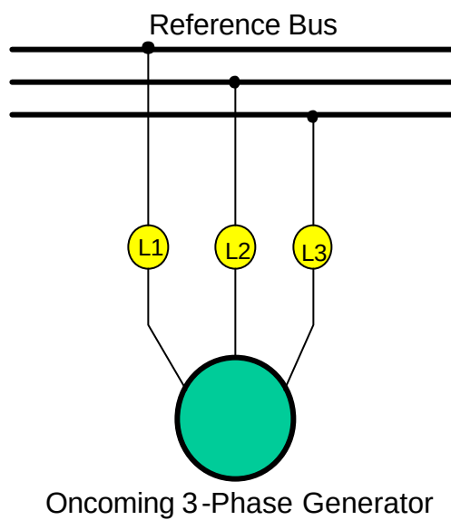
Figure 3: The Lamp Method Synchronization Circuit for a 3-Phase System [1]
