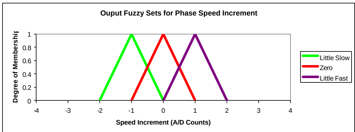
Figure 18: Fuzzy Output Sets for Phase Speed Increment [11]
