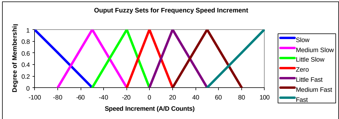
Figure 16: Output Fuzzy Sets for Frequency Speed Increment [11]
