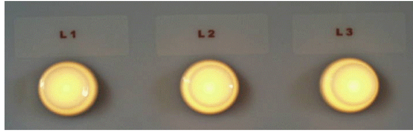
Figure 2: Lamps for 3-Phase Generator Synchronization [1]
