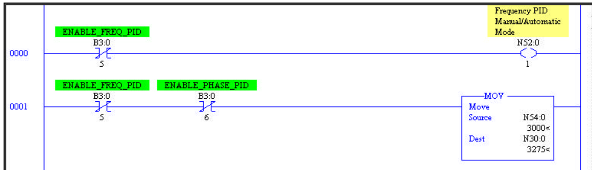
Figure 28: Ladder Logic Used to Startup the Prime Mover
