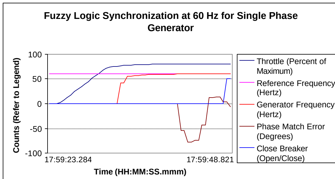
Figure 42: Fuzzy Logic Synchronization at 60 Hz for Single Phase Generator
