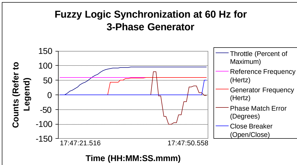
Figure 39: Fuzzy Logic Synchronization at 60 Hz for 3-Phase Generator
