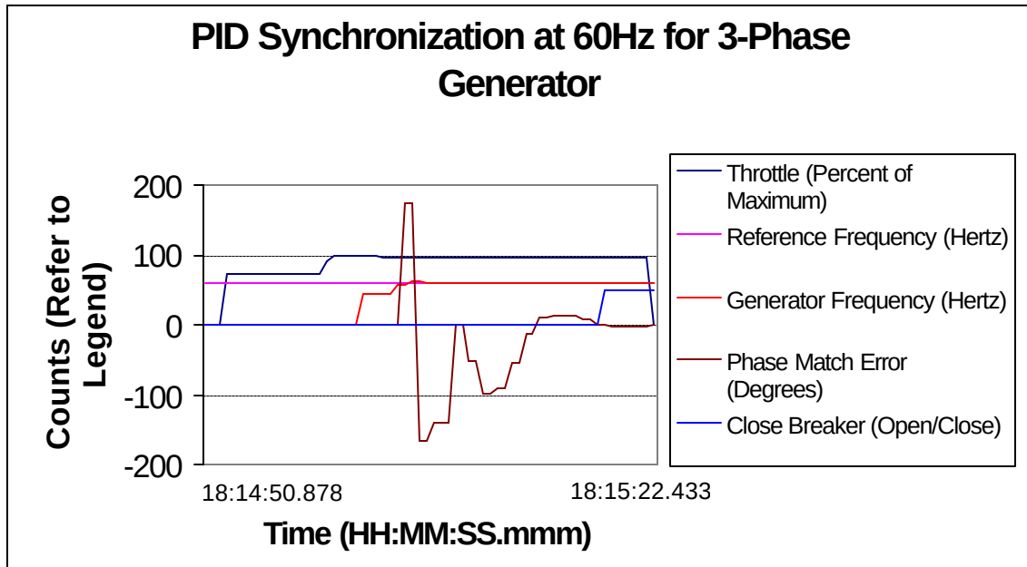
Figure 38: PID Synchronization at 60 Hz for 3-Phase Generator
