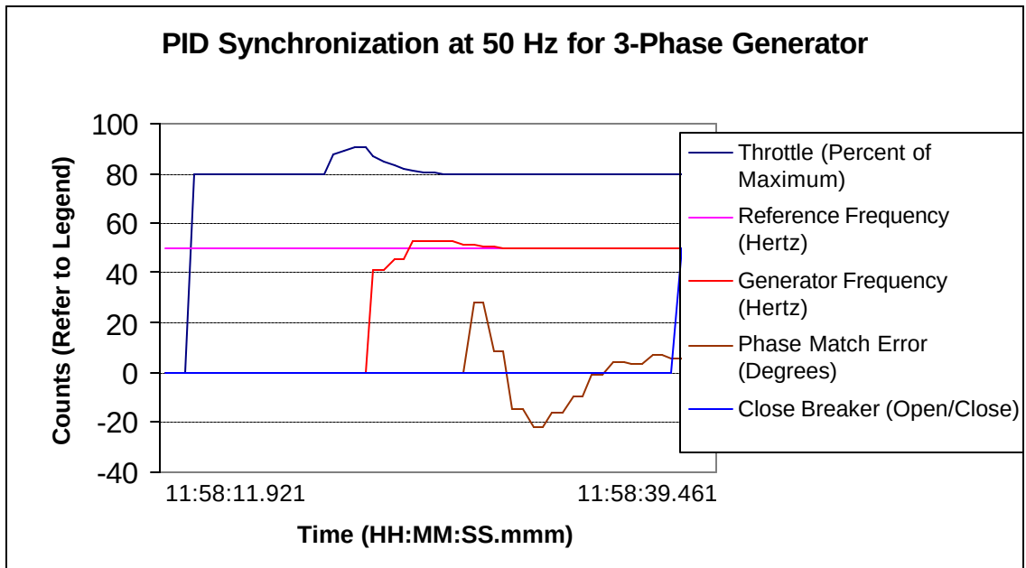
Figure 45: PID Synchronization at 50 Hz for 3-Phase Generator
