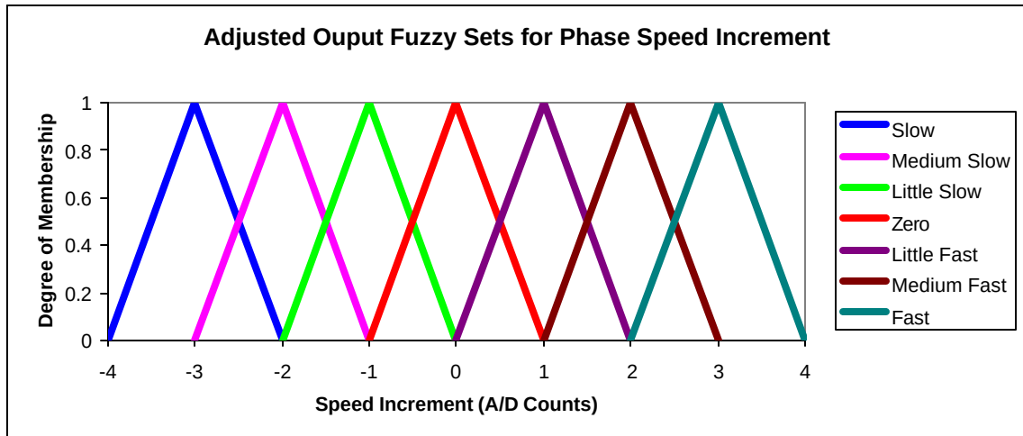
Figure 26: Adjusted Output Fuzzy Sets for Phase Speed Increment
