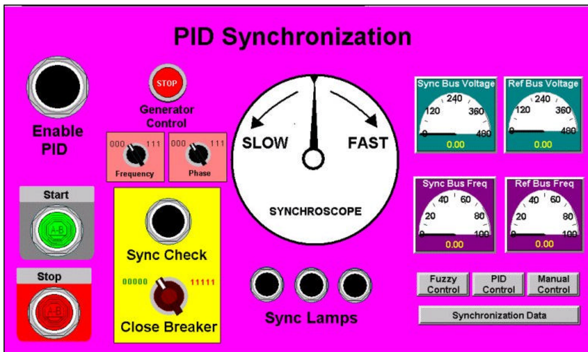
Figure 34: RSView32 Screen Used to Execute PID Synchronization
