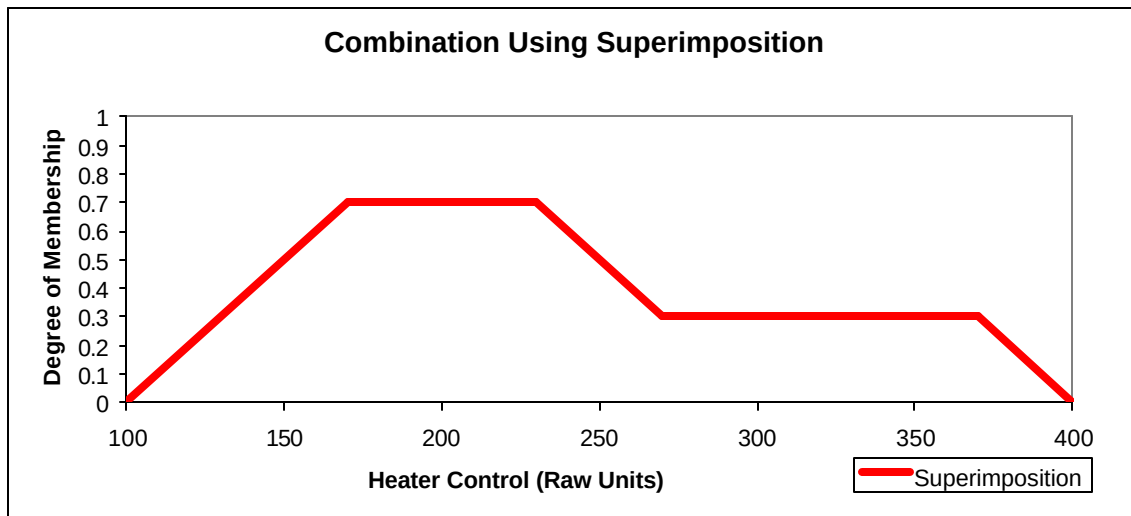
Figure 10: Combination Using Superimposition
