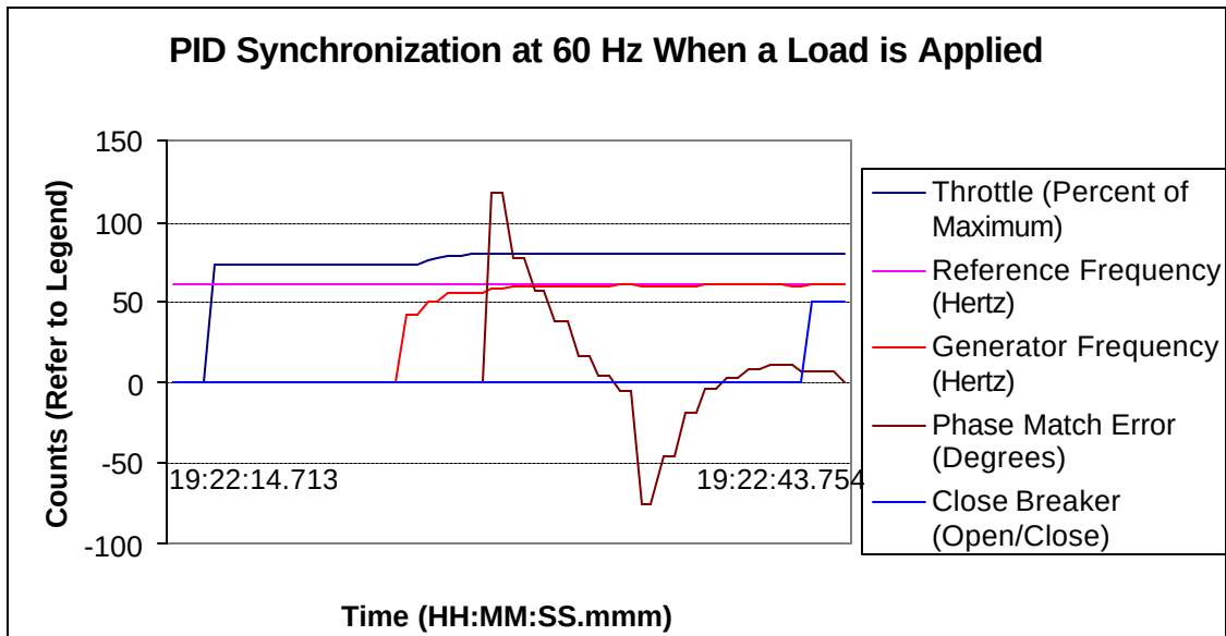
Figure 46: PID Synchronization at 60 Hz When a Load is Applied
