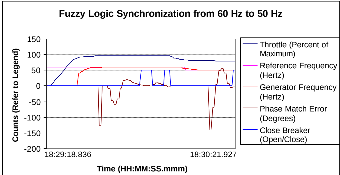
Figure 43: Fuzzy Logic Synchronization from 60 Hz to 50 Hz
